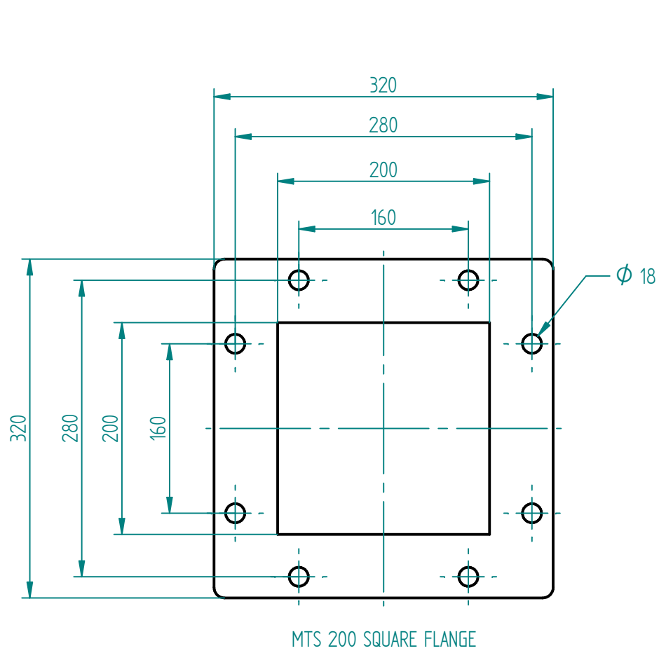
MTS 200 SQUARE FLANGE
