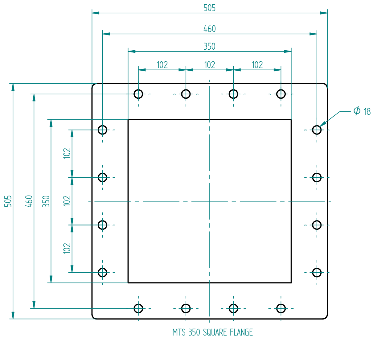
MTS 350 SQUARE FLANGE
