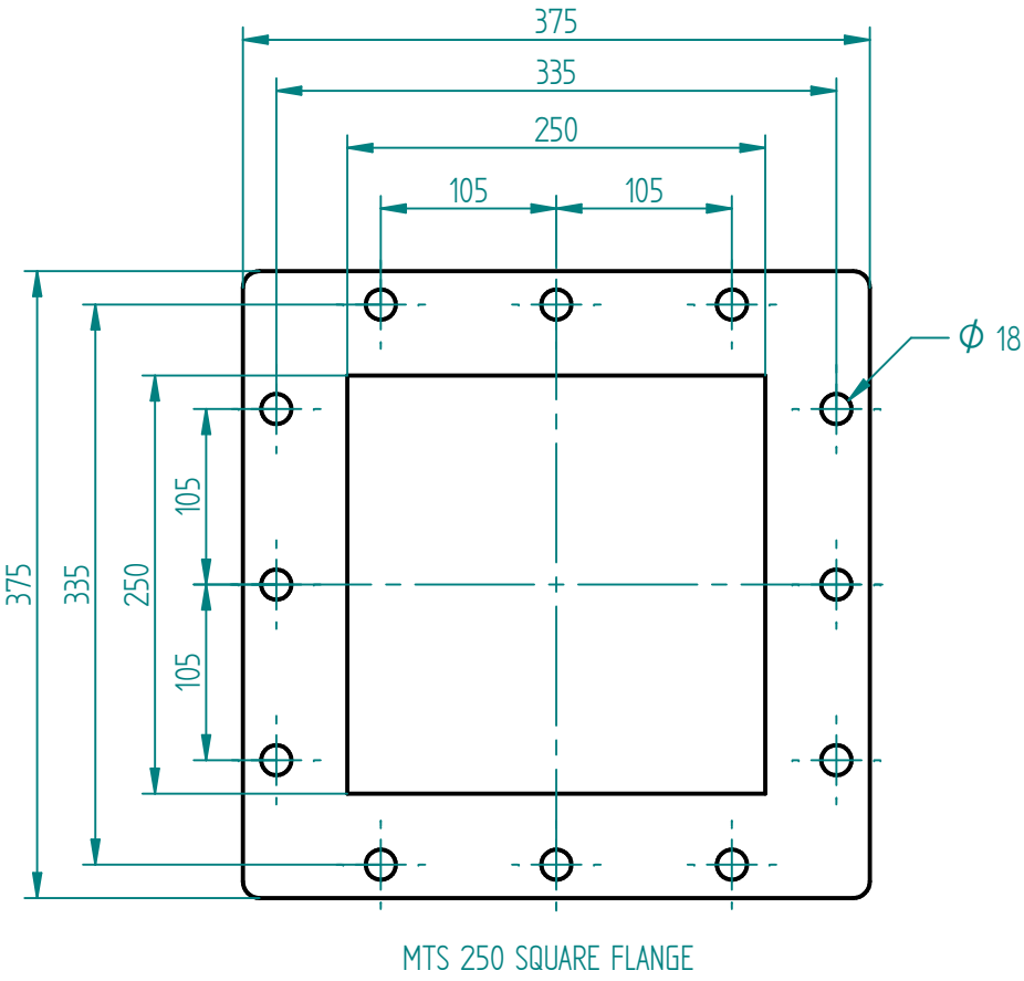
MTS 250 SQUARE FLANGE
