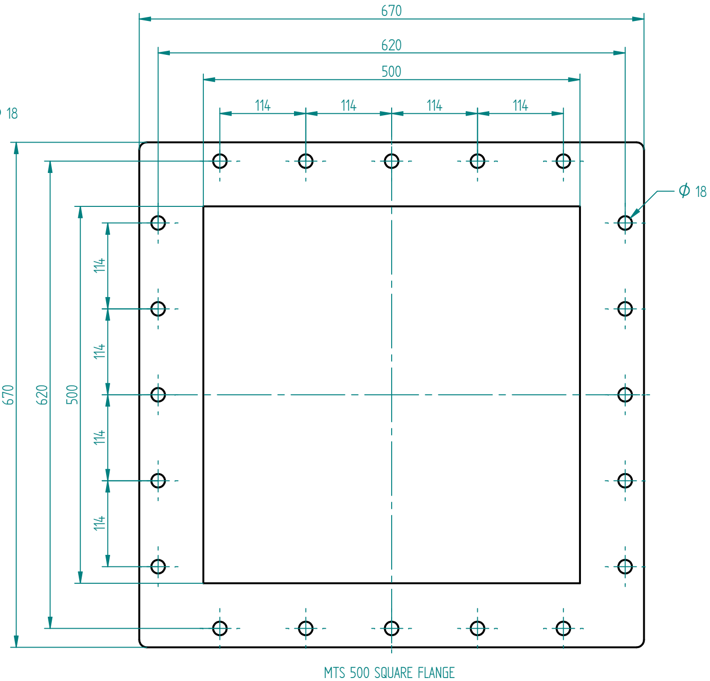
MTS 500 SQUARE FLANGE
