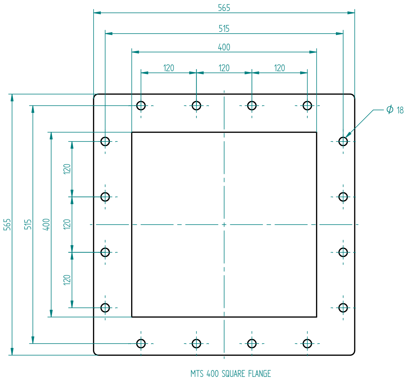
MTS 400 SQUARE FLANGE
