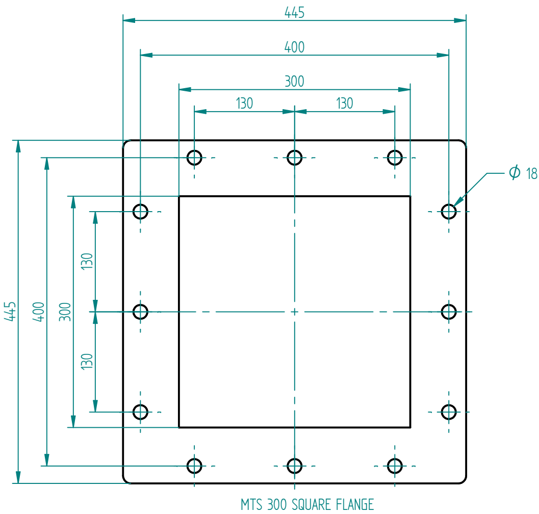
MTS 300 SQUARE FLANGE
